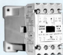
Side aux. Block Mechanical Interlock
